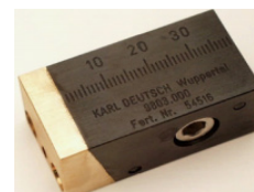
FLUXA 试块
